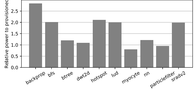
Figure 6: Normalized maximum power of 700 MHz relative to high power target (43 W).
