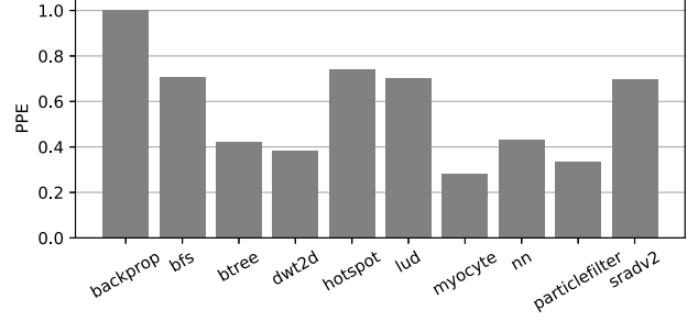
Figure 2: Optimal provisioned power utilization at 700 MHz across several rodinia benchmarks.
