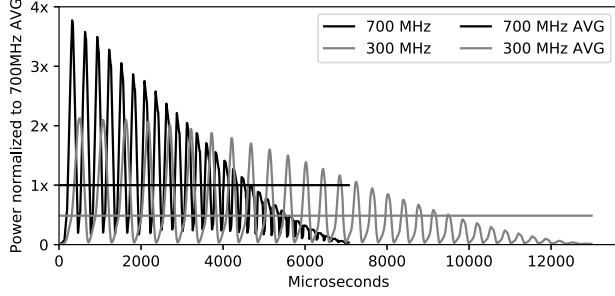
Figure 1: Normalized power over time of 300 MHz and 700 MHz GPU running LU Decomposition.
