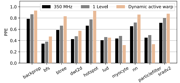
Figure 7: Provisioned power efficiency for the 43W power target.
